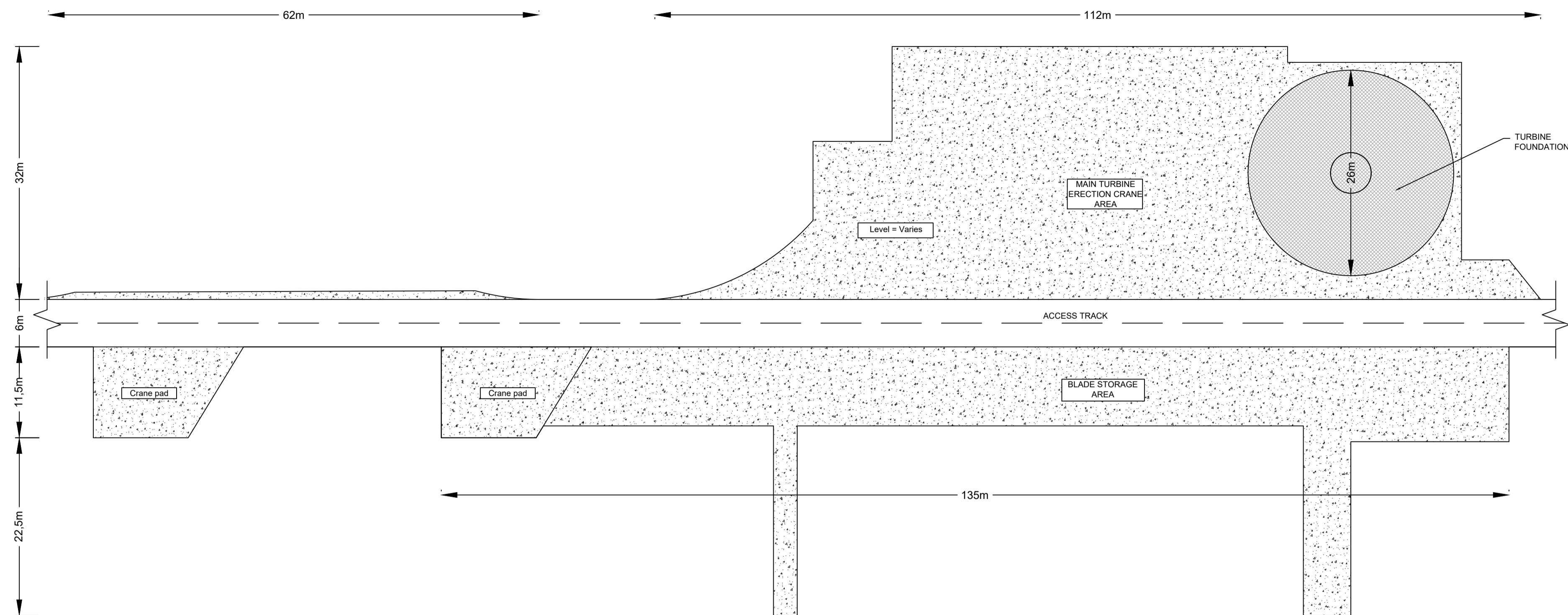
TURBINE HARDSTAND - LAYOUT PLAN SCALE 1:400
