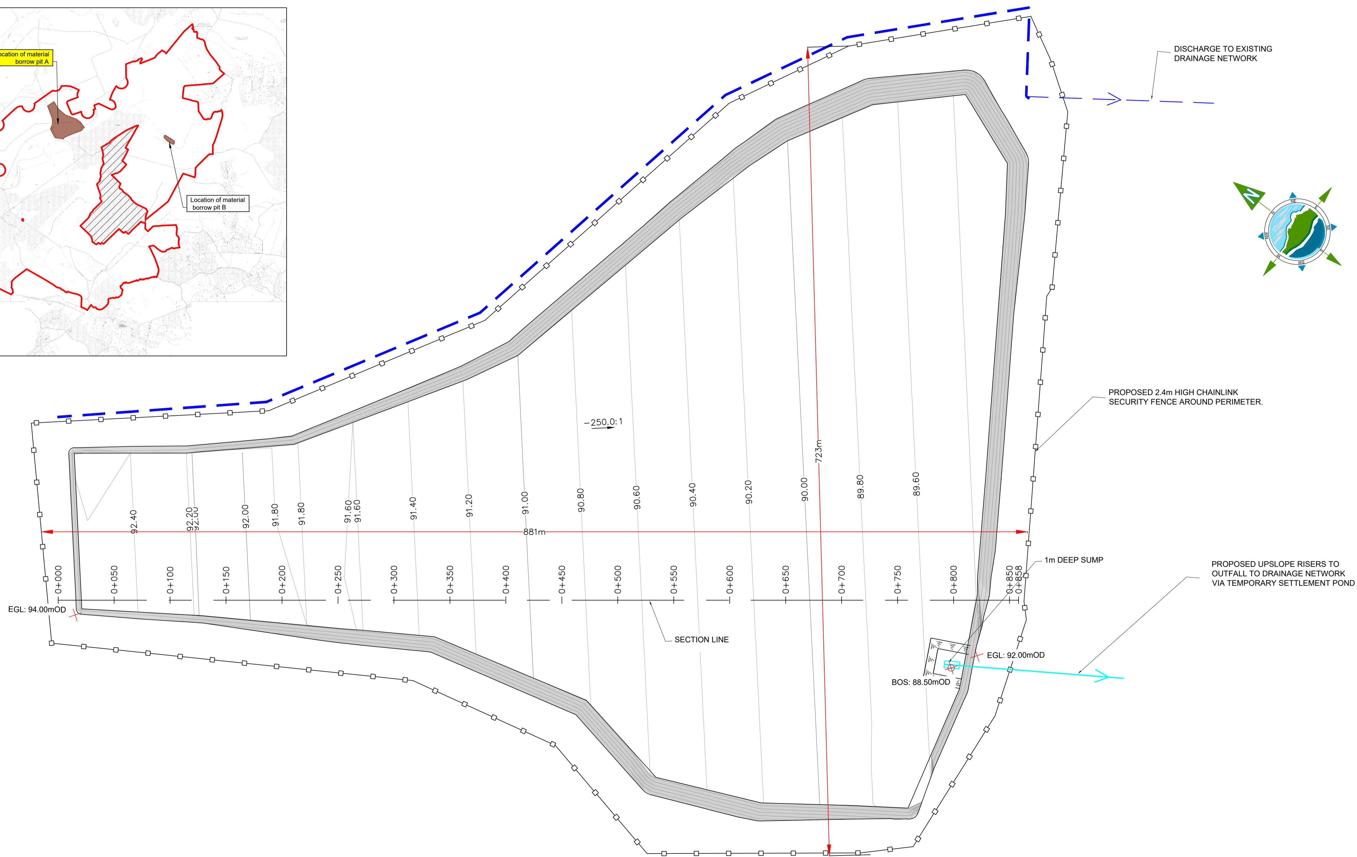
PLAN ON BORROW PIT Scale 1:2,000
